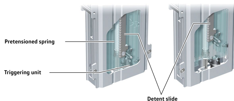
Automatic Rollover Support System not triggered
