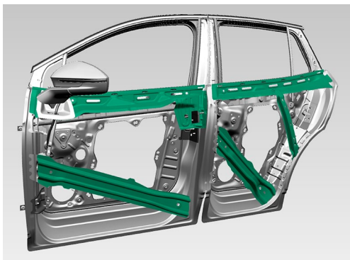
Side impact protection in the doors
